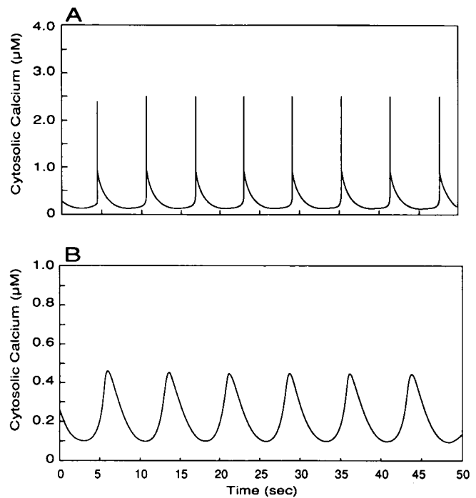
FIGURE 9 Simulation of the calcium oscillations with different concentrations of calcium binding sites: (A) 80 \mu\text{M} and (B) 140 \mu\text{M} . Note that with increased buffer the oscillations have a decreased amplitude and frequency.
