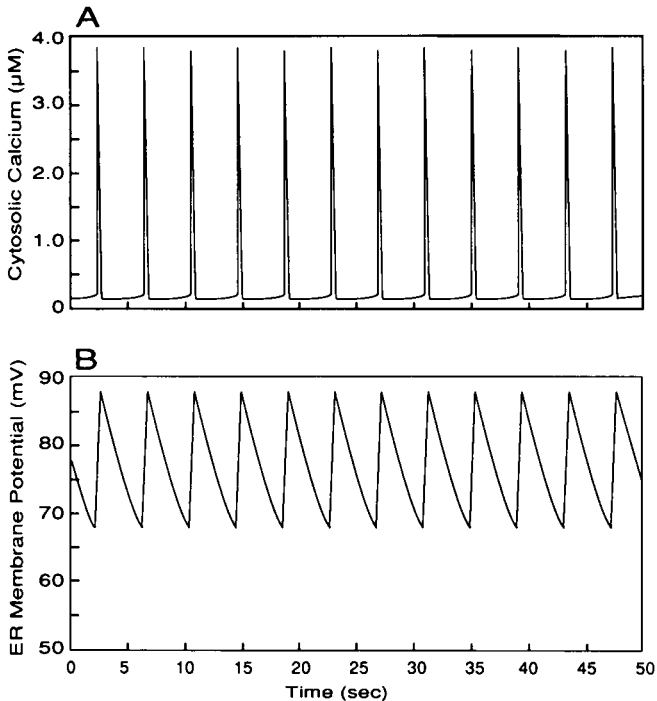
FIGURE 8 Simulation of the oscillations in (A) [\text{Ca}]_{\text{cyt}} and (B) ER membrane potential after removal of the buffer ( P_{\text{total}} = 0 , k_{\text{on}} = 0 , and k_{\text{off}} = 0 ). Note the increase in the amplitude and frequency of the oscillations.
