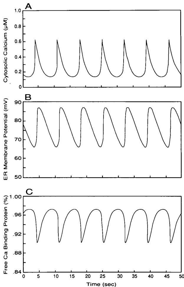
FIGURE 5 Simulation of intracellular calcium injection induced oscillations of (A) [Ca]_{cyt} , (B) ER membrane potential, and (C) percentage free calcium binding sites on calcium binding protein for a small constant flux of calcium into the cytosol ( q = 3.21 \times 10^{-10} \mu\text{mol/s} ).
